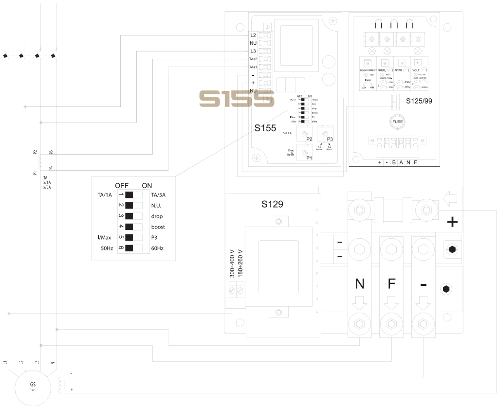
PIC. 3: Connecting diagram between an S155 Reactive Power Sharer and a S099 AVR
