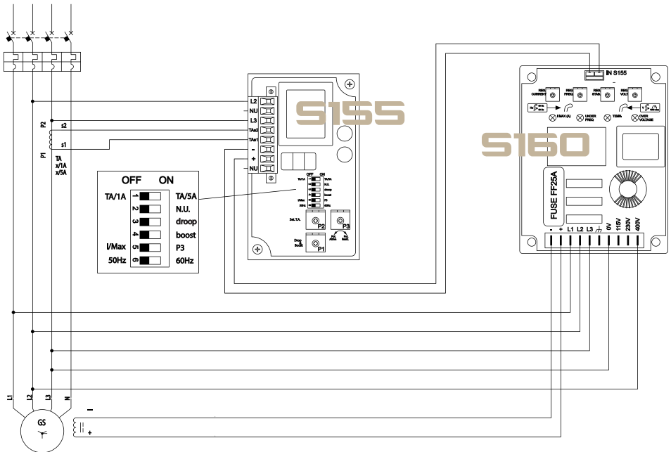
PIC. 1: Connecting diagram between an S155 Reactive Power Sharer and a S160 AVR
