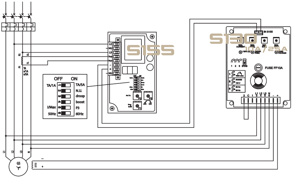
PIC. 1: Connecting diagram between an S155 Reactive Power Sharer and a S130 AVR
